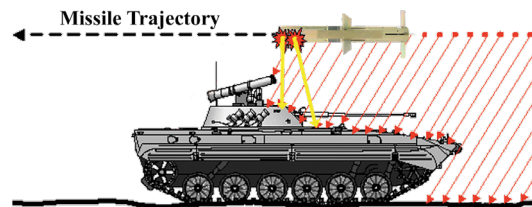
Toophan 3-M
